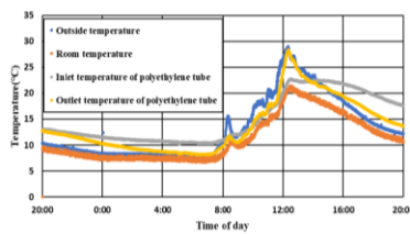
Air and water temperature
