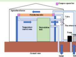
Structure of experimental apparatus
